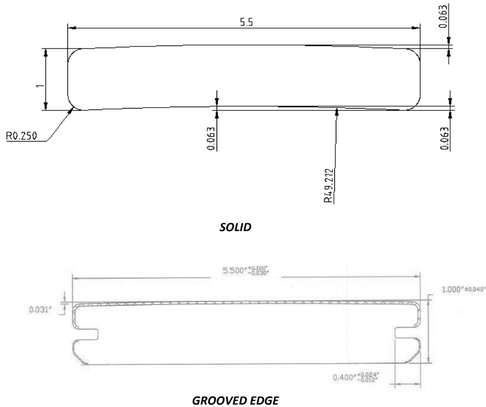
FIGURE 1 – VEKADECK™ DIMENSIONS
